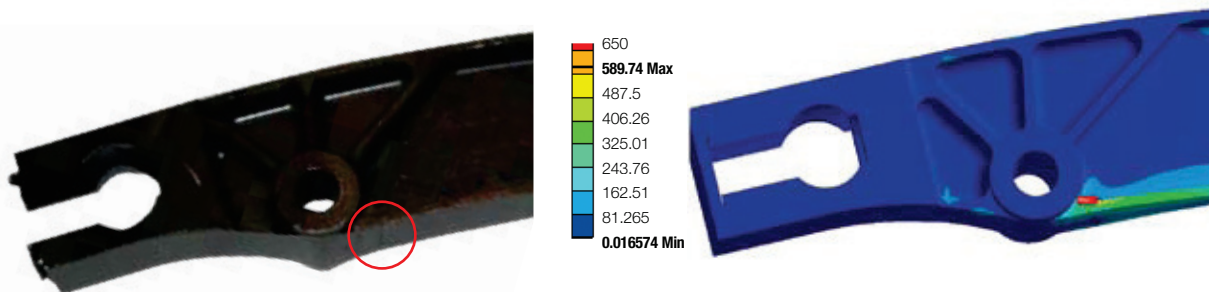
Brake pedal crack with simulation of equivalent stresses
