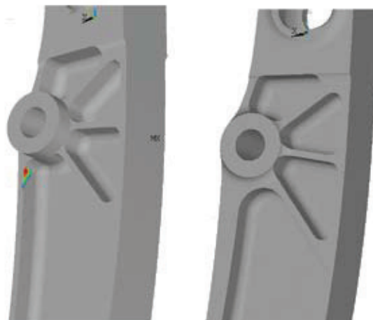
Original design in fe-safe (left) and redesigned component (right)
